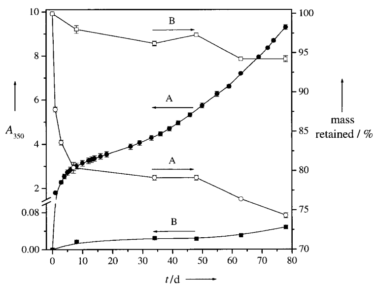
Figure 2. Dissolution of pressed pellets of poly- 1 (A) and poly- 2 (B), as monitored by solution UV/Vis absorbance ( \bullet , \blacksquare ) and mass loss ( \circ , \square ).
